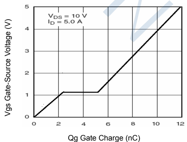
Figure 6 Gate Charge
