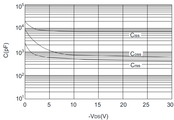
Figure 5 : Capacitance Characteristics
